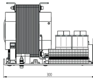
Outline Dimensions (mm(inch))
