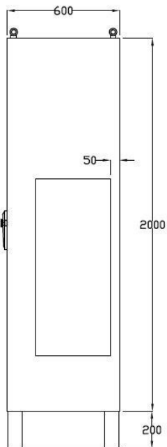
Outline Dimensions (mm(inch))
