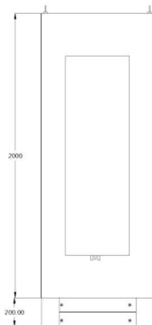
Outline Dimensions (mm(inch))
