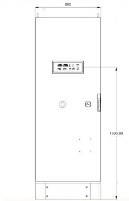
Outline Dimensions (mm(inch))
