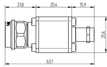
Outline Dimensions (mm(Inch))
