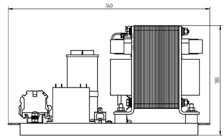
Outline Dimensions (mm(inch))
