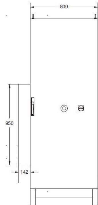
Outline Dimensions (mm(inch))
