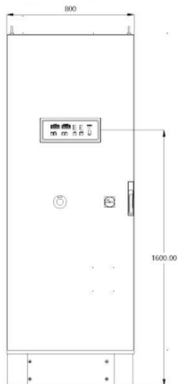
Outline Dimensions (mm(inch))
