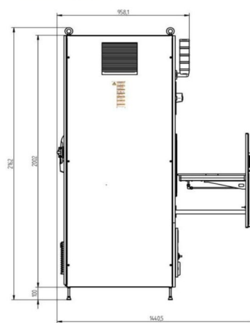
Outline Dimensions (mm(inch))
