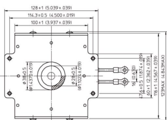
Tube Outline Dimensions (mm(inch))
