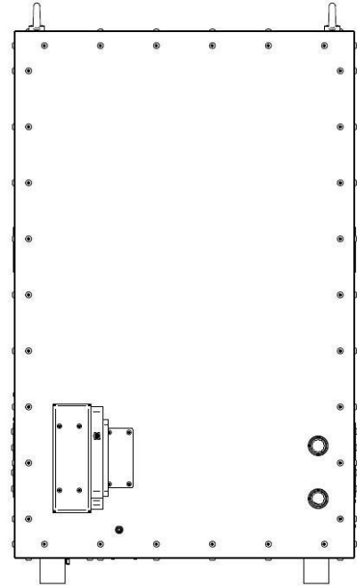
Outline Dimensions (mm(inch))
