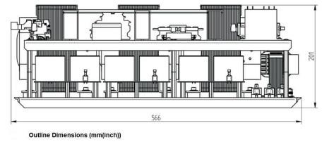
Outline Dimensions (mm(inch))
