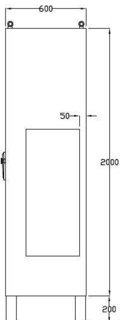
Outline Dimensions (mm(inch))
