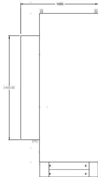
Outline Dimensions (mm(inch))
