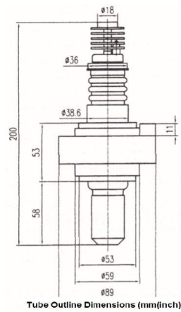
Tube Outline Dimensions (mm(inch))
