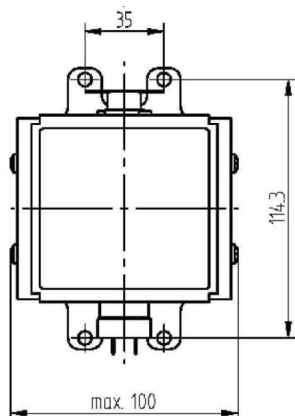
Tube Outline Dimensions (mm(inch))
