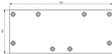
Outline Dimensions (mm(inch))
