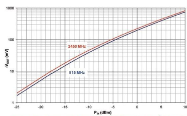
Typical transfer characteristic (f = 915 MHz and 2450 MHz, RLOAD = 33 kΩ, TA = 25 °C)
