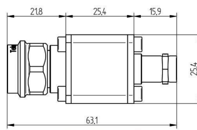
Outline Dimensions (mm(Inch))
