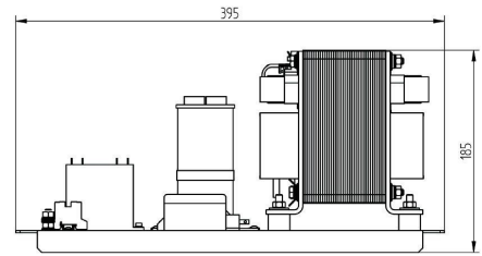
Outline Dimensions (mm(inch))
