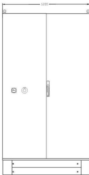
Outline Dimensions (mm(Inch))
