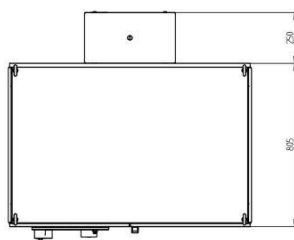
Outline Dimensions (mm(inch))
