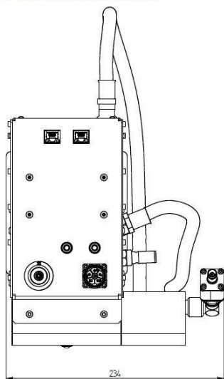
Outline Dimensions (mm(inch))
