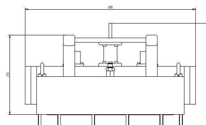
Outline Dimensions (mm(inch))
