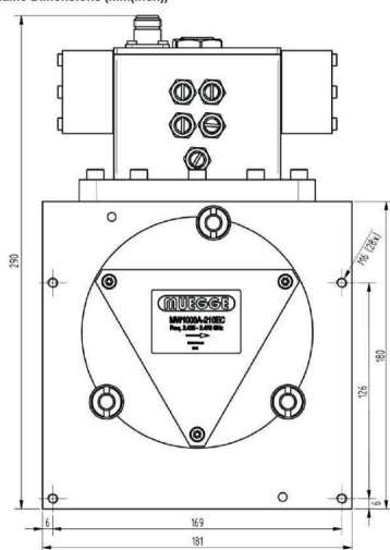
Outline Dimensions (mm(inch))
