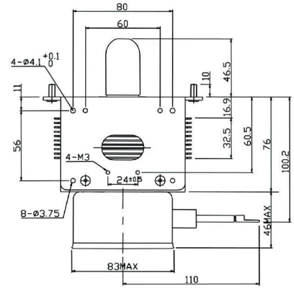
Tube Outline Dimensions (mm(Inch))
