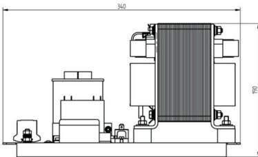
Outline Dimensions (mm(inch))
