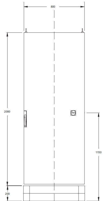
Outline Dimensions (mm(inch))
